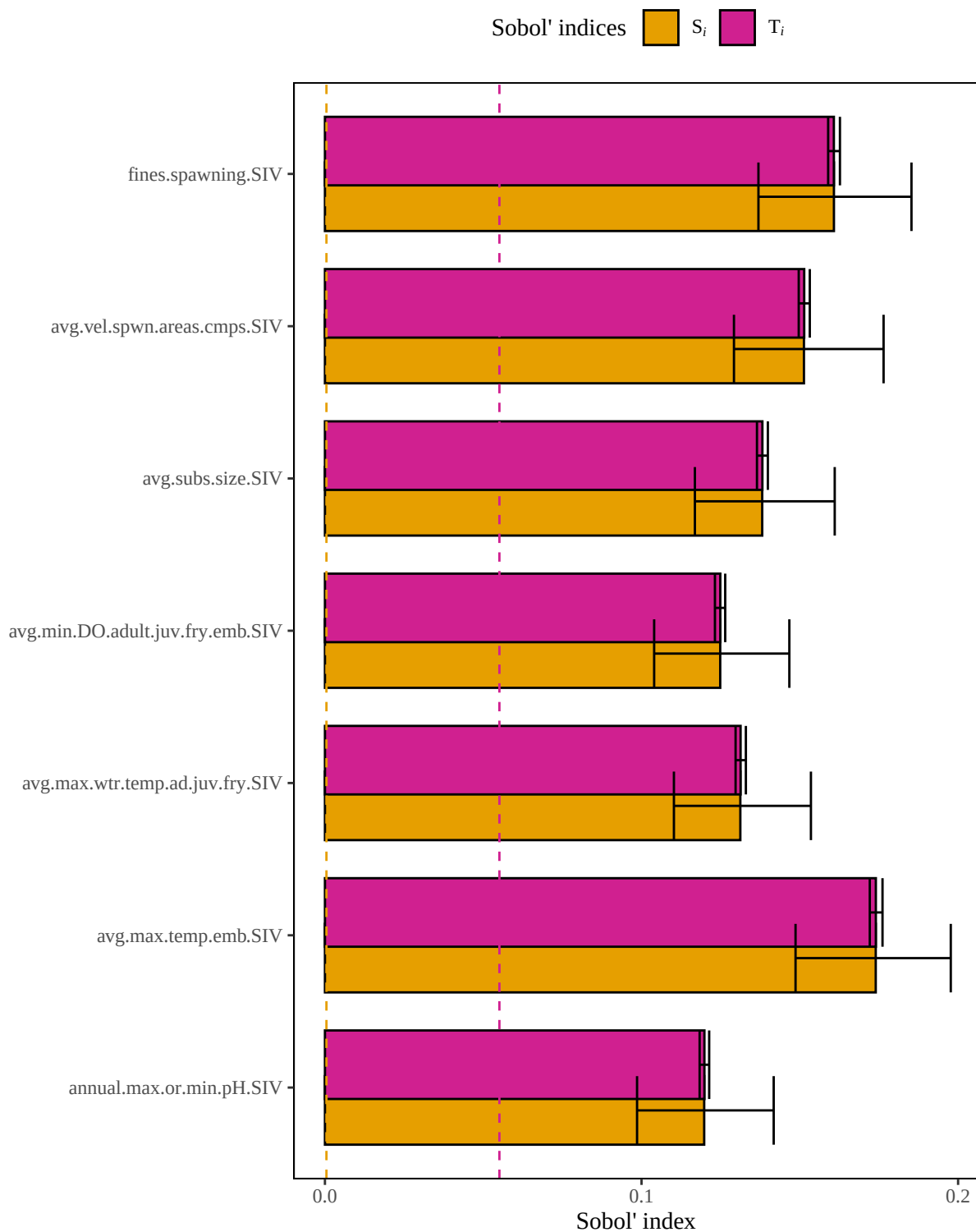
Figure 4. Results of a sensitivity analysis for the cutthroatLacLahontanLtoe15C model based on an arithmetic mean structure. Dashed lines represent baseline numerical approximation error for S_i and T_i ( i.e. , dummy variables).
