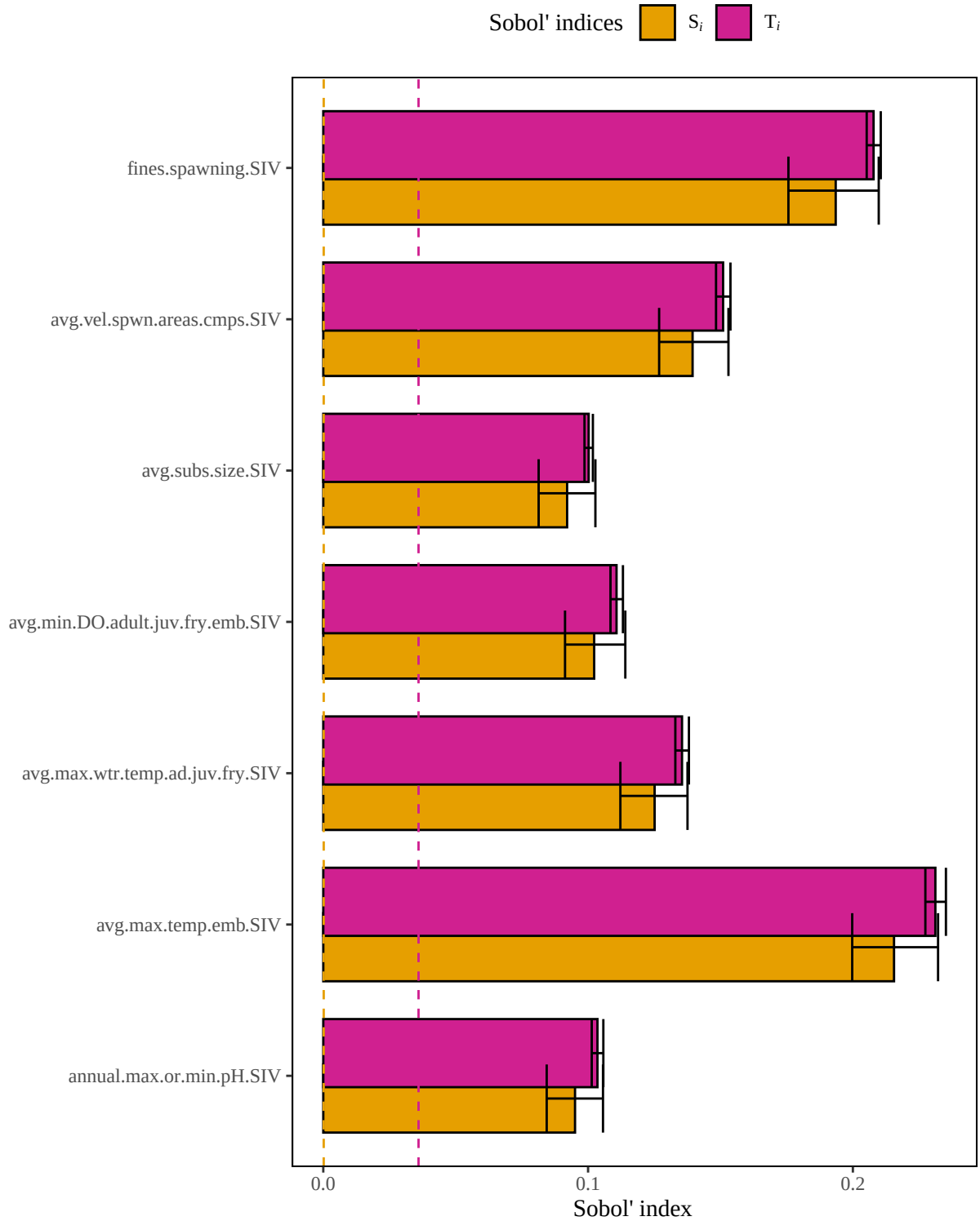
Figure 5. Results of a sensitivity analysis for the cutthroatLacLahontanLtoe15C model based on a geometric mean structure. Dashed lines represent baseline numerical approximation error for S_i and T_i ( i.e. , dummy variables).
